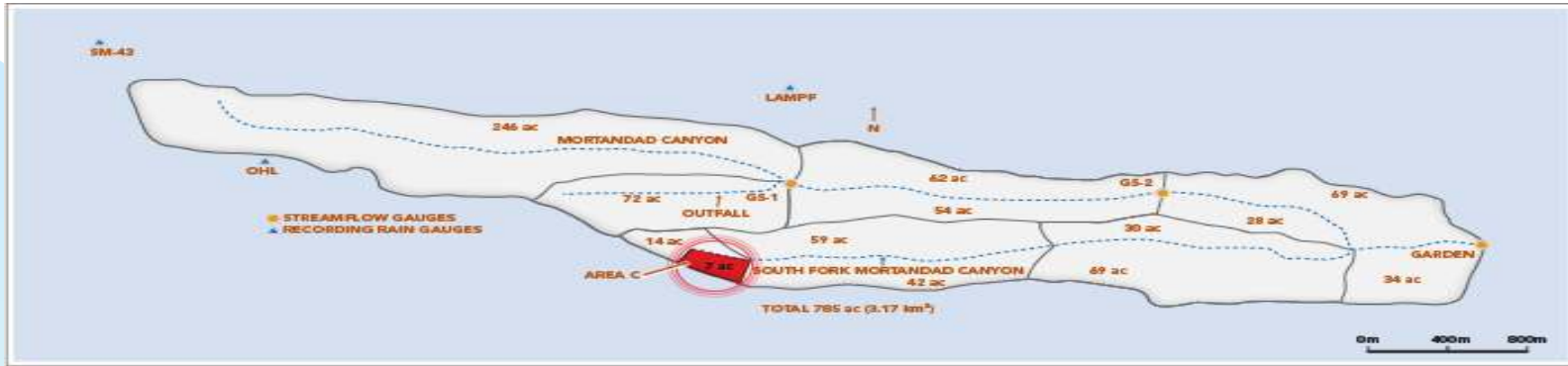
Surface Runoff
