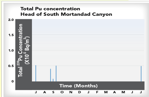
Total Pu (Sum of Dissolved and sorbed)
